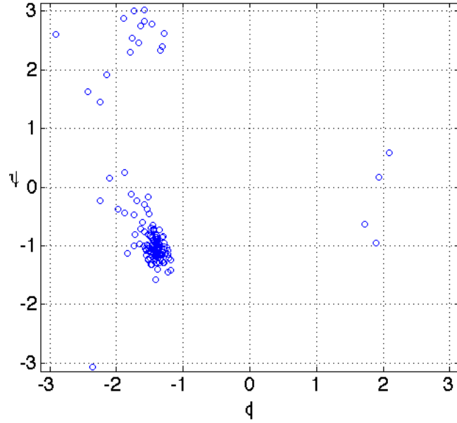
Figure 2.7. Ramachandran plot for the protein molecule with PDB identifier 5MBA.
