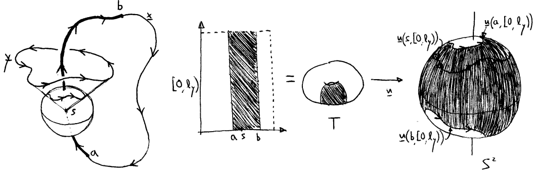
Figure D.2. When \mathbf{x} passes through \mathbf{y} , the corresponding section of the torus T collapses around the unit sphere S^2 .
