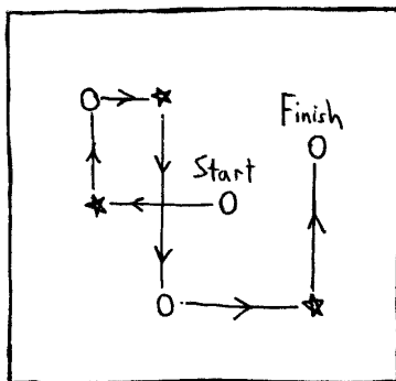
Figure B.1. Tendril terminating at a 0 with no ★ in its row.
