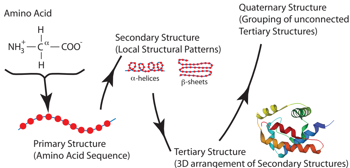
Figure 7.1. Proteins exhibit a hierarchy of organizational levels.
