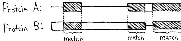
Figure 7.4. Structurally similar proteins usually have corresponding pieces that are in the same order and direction.
