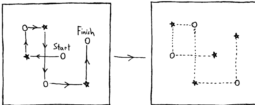
Figure B.2. We end with one more ★ than when the core routine started.
