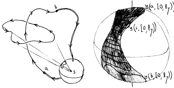
Figure D.3. When \mathbf{x} passes around the outside of \mathbf{y} , the corresponding section of the torus T is squashed onto one side of the unit sphere S^2 .
