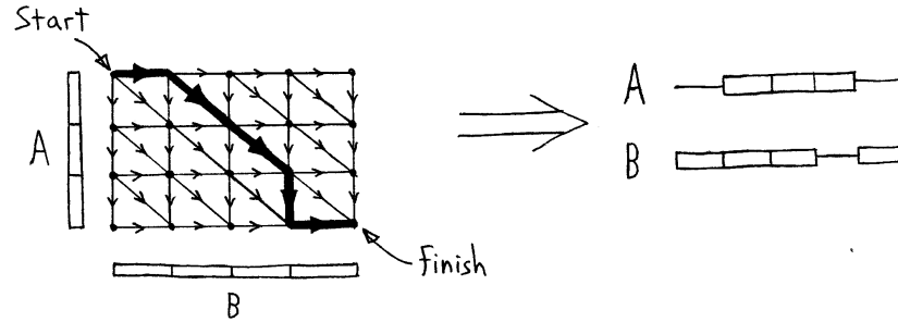
Figure C.1. Rectangular grid of nodes.
