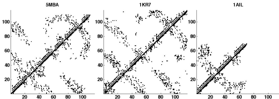
Figure 7.6. D-sets for three of the molecules from Section 7.2, with r = 15\text{\AA} . Axes are in units of residues.
