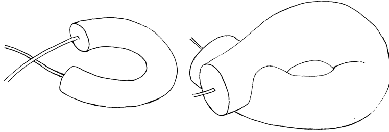
Figure 4.4. Singularities arise in the tube \mathcal{D} associated with a space curve as the tube radius r increases. Recall (see 2.2) that the curve global injectivity radius r_i is the largest radius value for which \mathcal{D} is singularity free.
