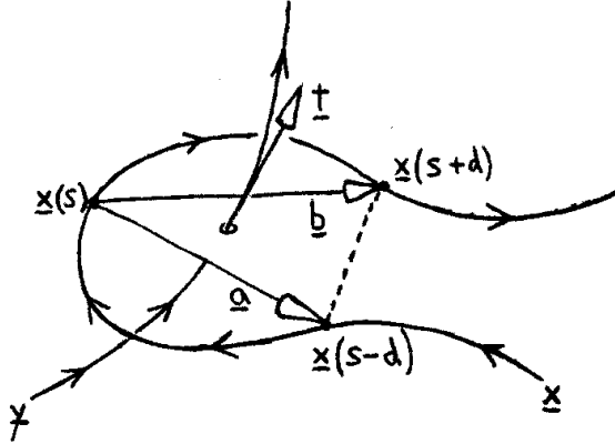
Figure 3.6. Diagram of vectors associated with (s, t) \in E_d .
