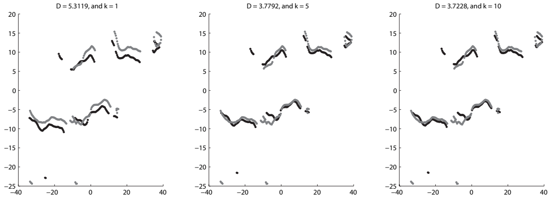
Figure 6.4. Algorithm translates two E-sets (from Figure 6.3) so that the distance D between them is minimized. We start the algorithm with the E-sets centered about the origin. The D values asymptote to approximately 3.72 Å.
