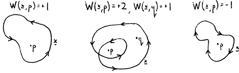
Figure 2.3. Examples of plane curves and their winding numbers.
